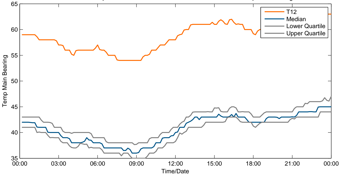
Outlier Unit Compared to Wind Farm Median and Quartile Values of Temp Main Bearing
